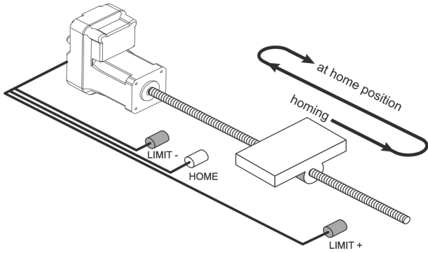
Figure 4: Open loop system with incremental encoder with typical homing sequence with linear motion axis, using one home and two limit sensors (Source: Schneider Electric)
