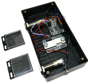
Figure 3: The miniature PLC processes the data and controls the display (Source: RS Components)
