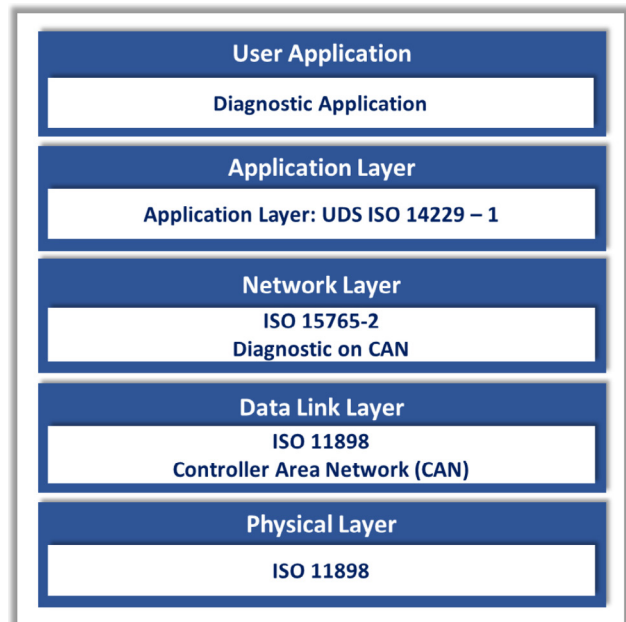
Figure 1: Architecture of UDS protocol (Source: iWave)
