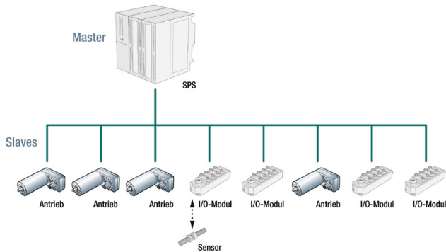
Figure 2 and Figure 3: before/after comparison - Thanks to the integrated intelligence, the drive can be freely programmed in a similar manner to a PLC, what offers the possibility of dispensing with a higher-level PLC (Photo: EBM-Papst)
